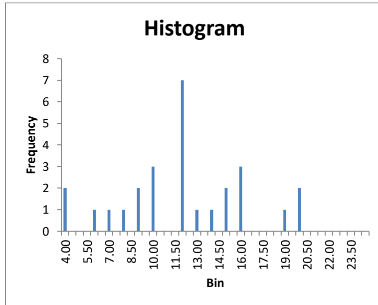
Figure 44. Sample histogram.
